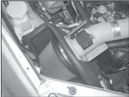
22. Slide the K&N® air filter onto the radiused adapter and secure with the provided hose clamp as shown.
