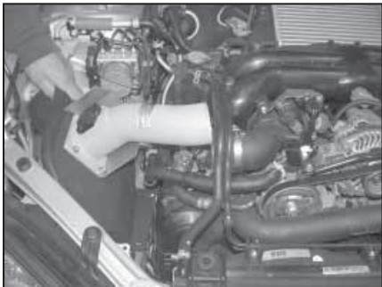
20. Install the complete assembly into the vehicle as shown.
