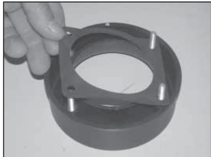
13. Apply one of the provided gaskets onto the adapter as shown.
