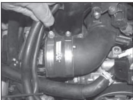
17. Install the provided silicone hose and hose clamps onto the turbo inlet tube as shown.
