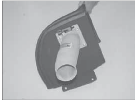
15. Install the intake tube onto the studs and secure with two of the provided nylock nuts and flat washers as shown in the orientation.
