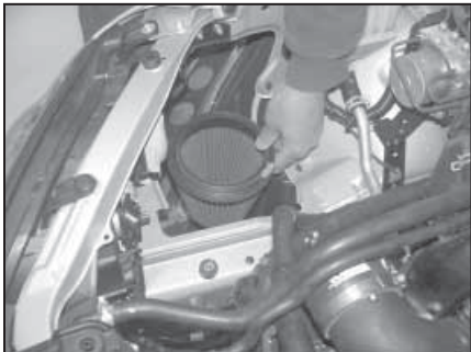
19. Place the K&N® air filter into the cavity in the inner fender as shown.
