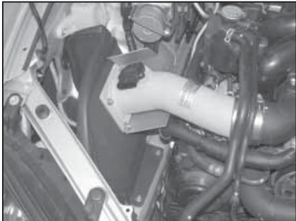
21. Line up the heat shield with the rubber mounted studs and secure with the provided nylock nuts, then, slide the intake tube into the silicone hose and secure as shown.
